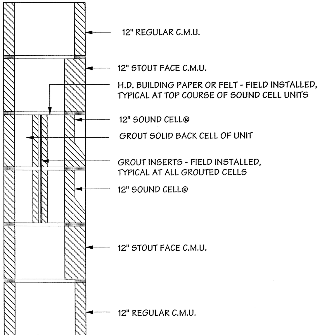
WALL SECTION SCALE : 1-1/2" = 1'-0"
