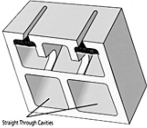
TYPE RSCRF (12")
